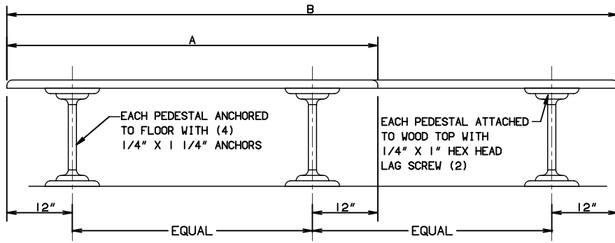
FRONT ELEVATION
