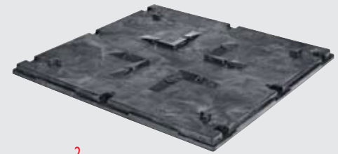
S Top Cap Model No. TV48450300 Dim: L 49" x W 46" x H 2.75" Construction: Vacuum Formed Color: Black
