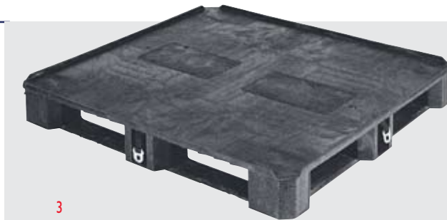
S Model No. PO48450632 (3) Dim: L 48" x W 45" x H 6** Color: Black
