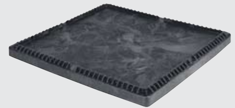
S Top Cap Model No. TV48450300 Dim: L 49.13" x W 46.13" x H 2.75" Construction: Vacuum Formed Color: Black
